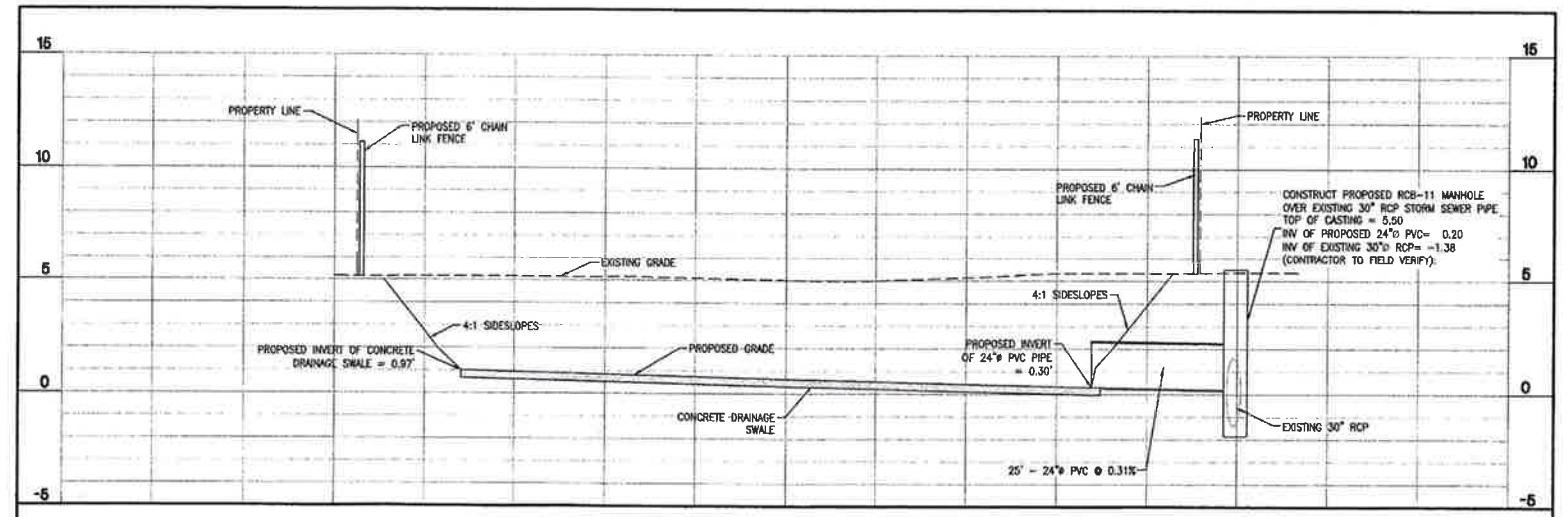
POND CROSS SECTION A-A
